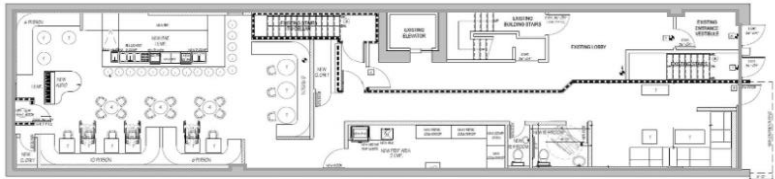
2 FIRST FLOOR CONSTRUCTION PLAN
